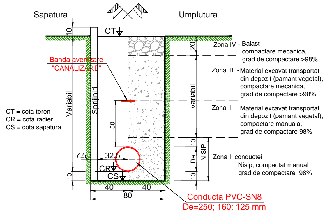
Detaliu pozare conducta gravitationala De= 250; 160; 125mm in zona drum nemodernizat
